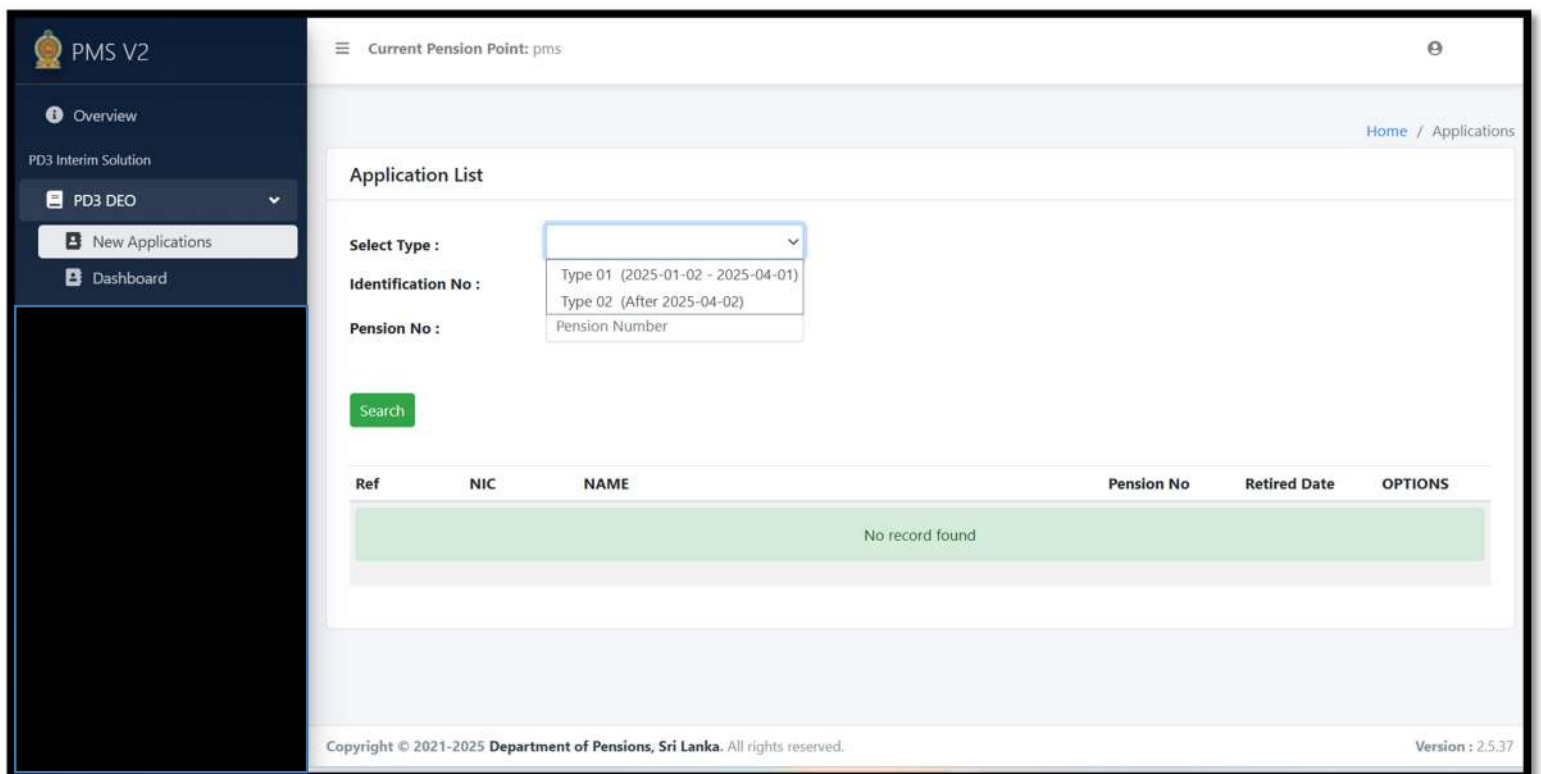
Figure 4. System Interface
