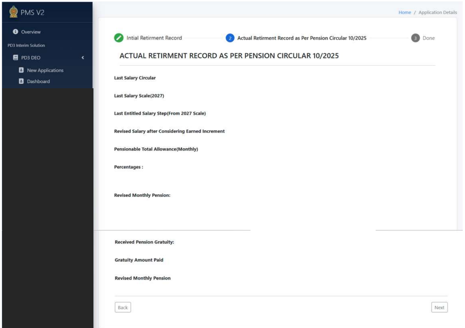
Figure 7.Application Interface I
