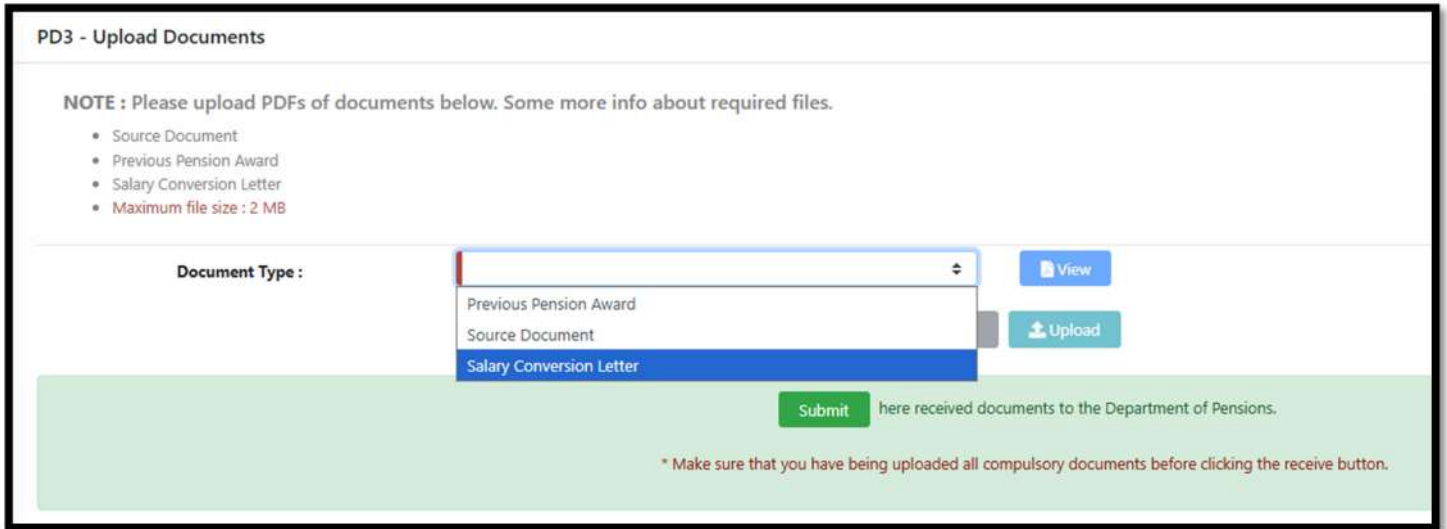
Figure 11.Document Upload View
